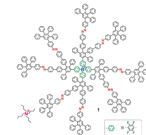
Scheme 1. Illustration of size and the density switching of a rigidly dendronized anion by azobenzene photoisomerization.
